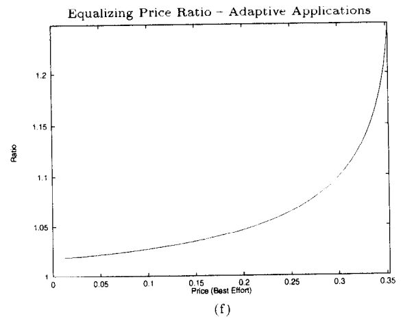
Figure 4: Algebraic Distribution - Utility, Bandwidth Gap, and Price Ratio to Equalize Welfare for Rigid and Adaptive Applications.
