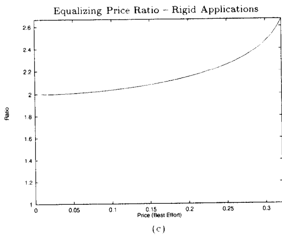
Figure 4: Algebraic Distribution - Utility, Bandwidth Gap, and Price Ratio to Equalize Welfare for Rigid and Adaptive Applications.
